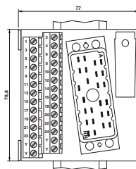
Чертеж UMK-EC56/25/EX-R
